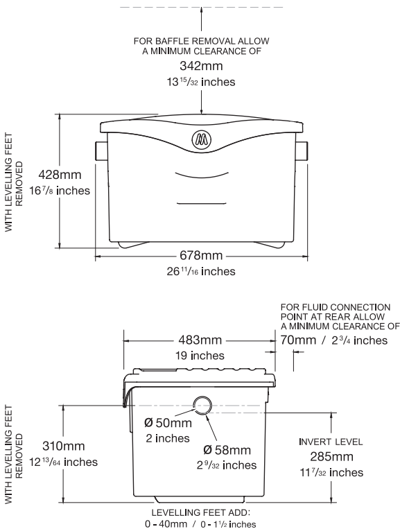
F.I.T UNIT (see separate data sheet for DOSING MODULE)
